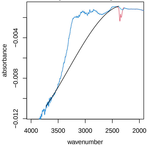
UTQ293 alkane region
