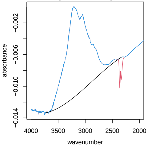
UTQ292 alkane region
