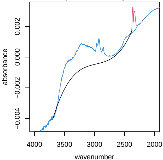
UTQ329 alkane region
