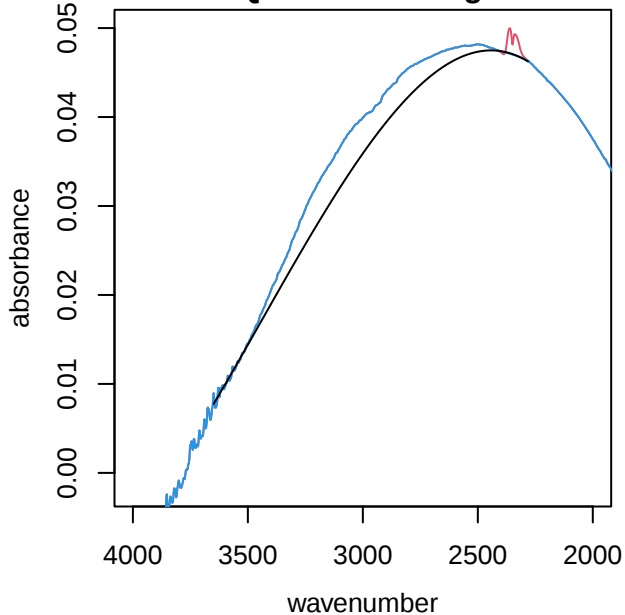
UTQ291 alkane region
