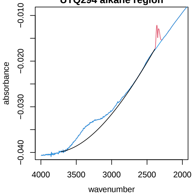
UTQ294 alkane region
