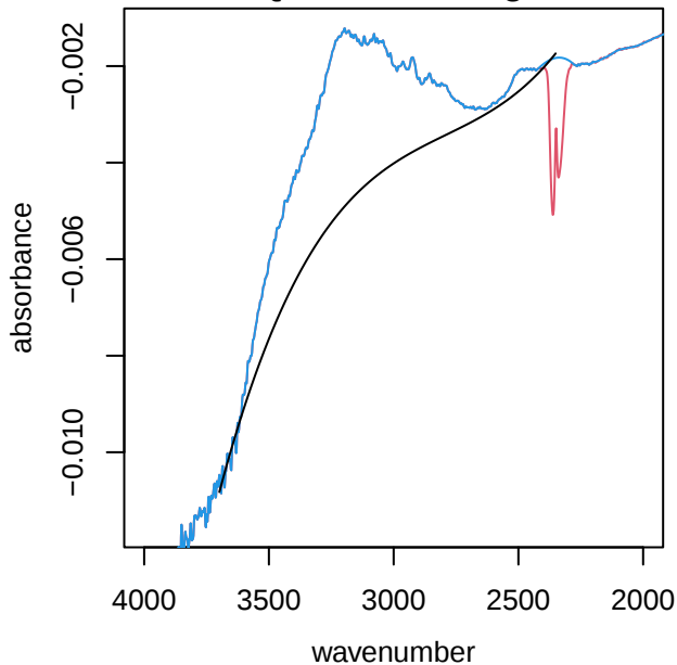
UTQ290 alkane region
