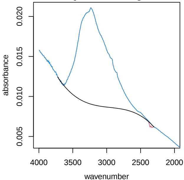
UTQ332 alkane region
