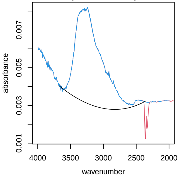
UTQ333 alkane region
