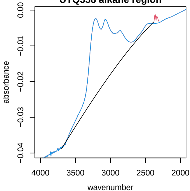
UTQ338 alkane region
