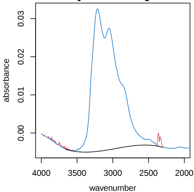
UTQ339 alkane region
