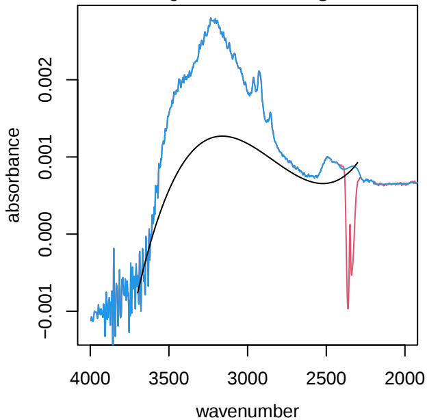
UTQ310 alkane region
