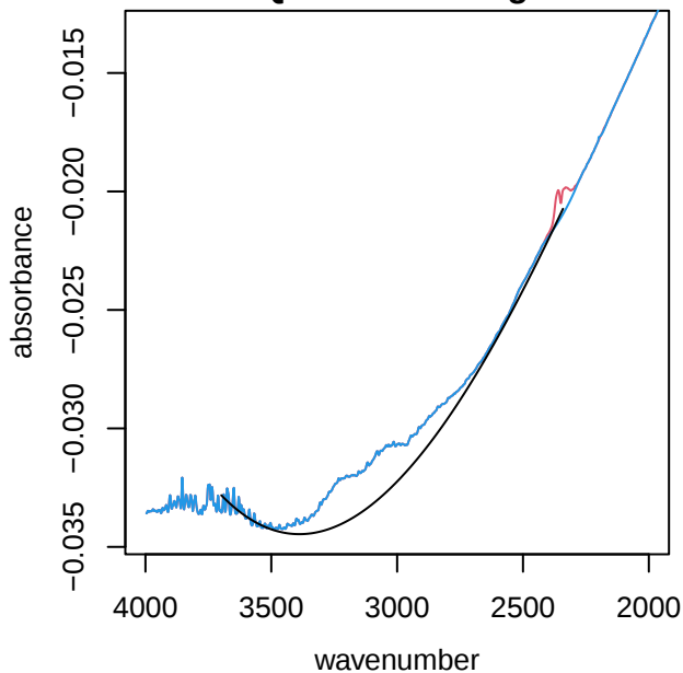
UTQ204 alkane region
