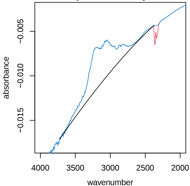
UTQ286 alkane region
