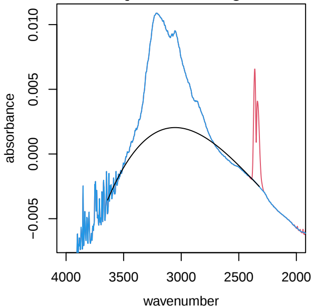
UTQ212 alkane region
