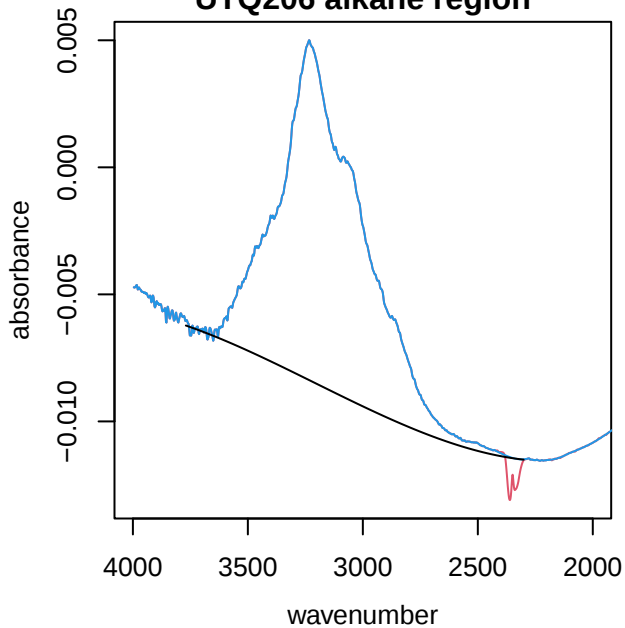
UTQ206 alkane region
