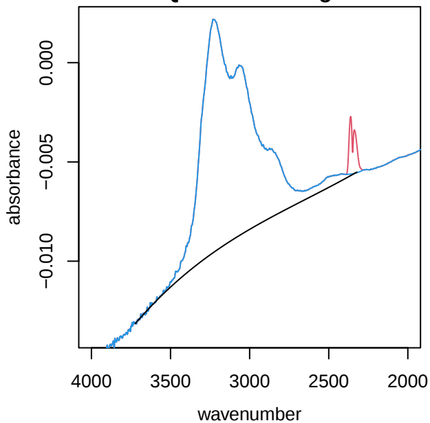
UTQ285 alkane region
