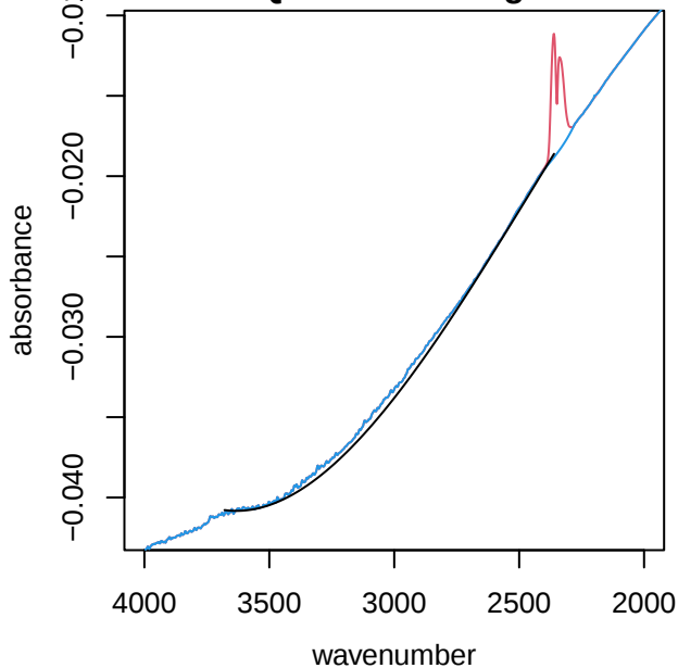
UTQ202 alkane region
