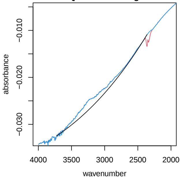
UTQ200 alkane region
