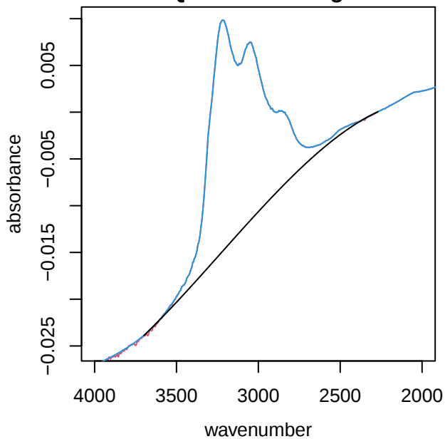
UTQ283 alkane region
