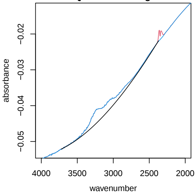
UTQ213 alkane region
