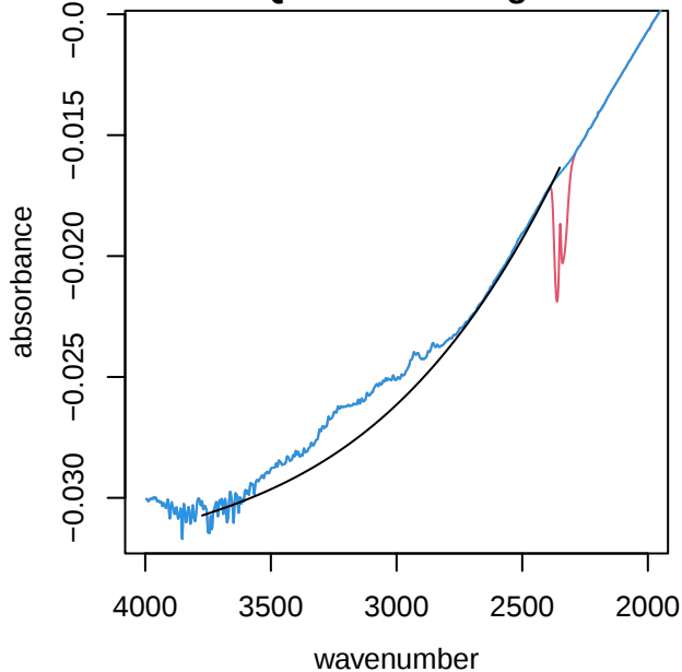
UTQ201 alkane region
