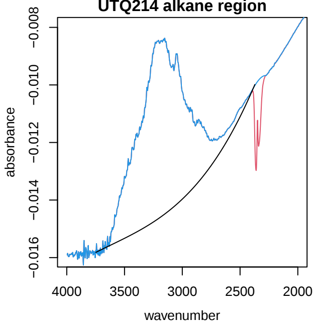
UTQ214 alkane region
