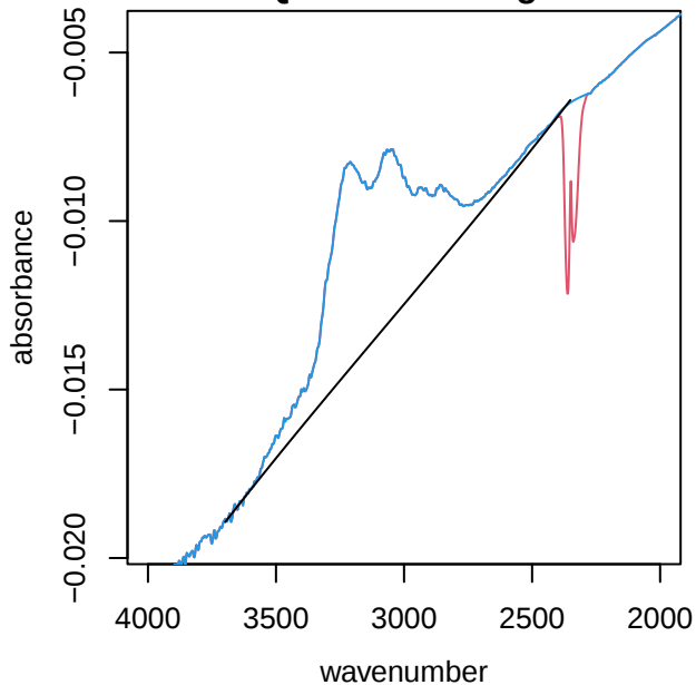
UTQ203 alkane region
