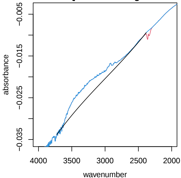
UTQ296 alkane region
