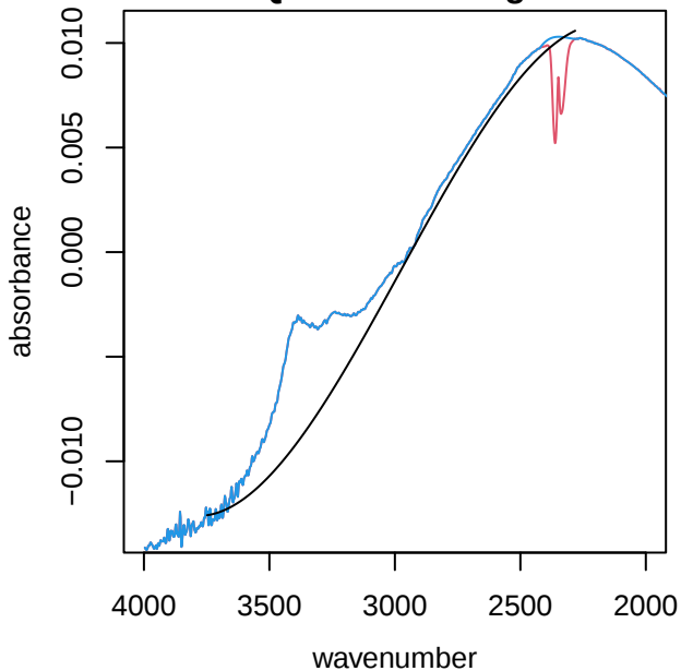
UTQ320 alkane region
