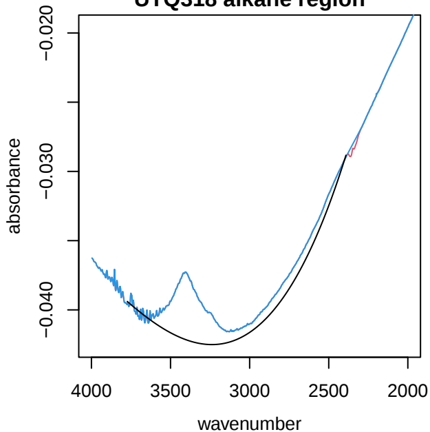
UTQ318 alkane region
