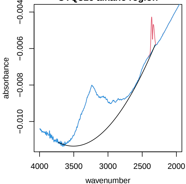
UTQ316 alkane region
