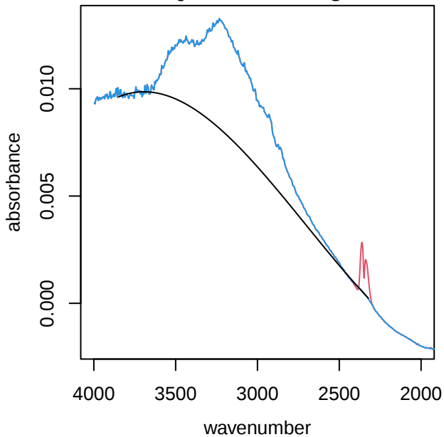
UTQ299 alkane region
