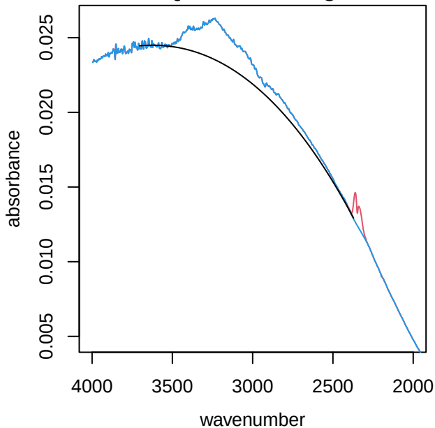
UTQ297 alkane region
