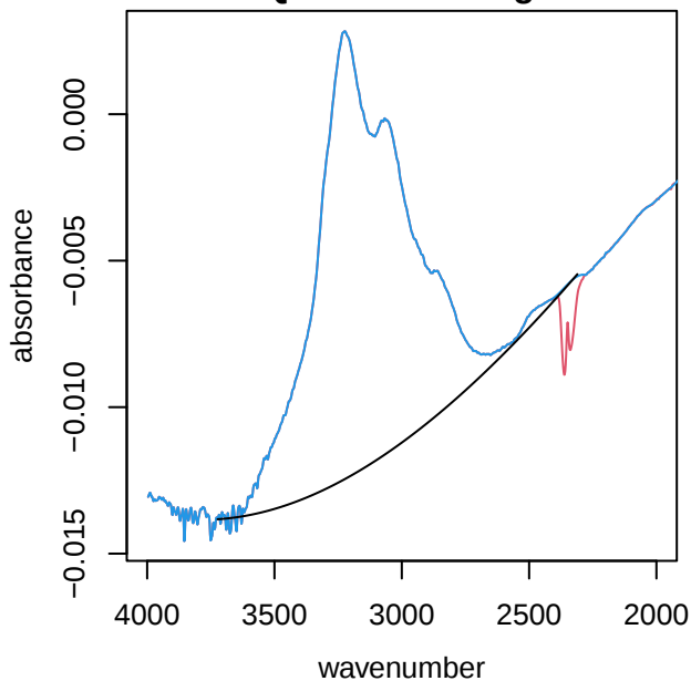
UTQ314 alkane region
