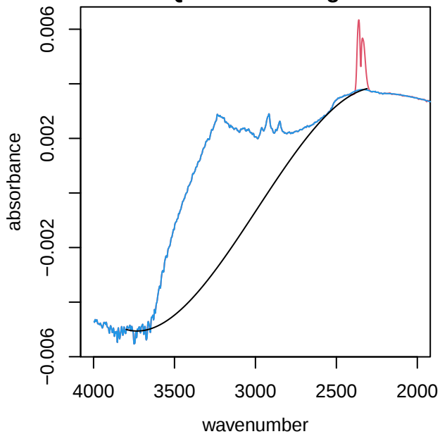
UTQ315 alkane region
