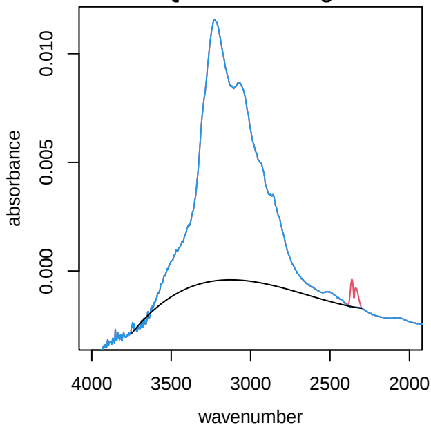
UTQ241 alkane region
