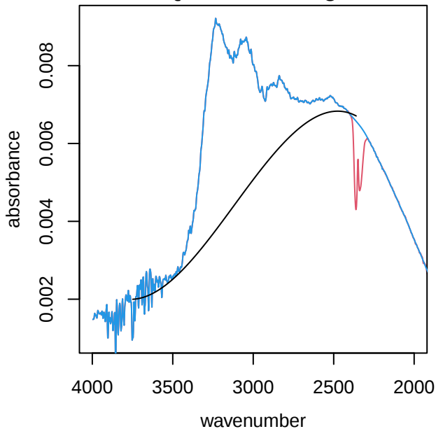
UTQ245 alkane region
