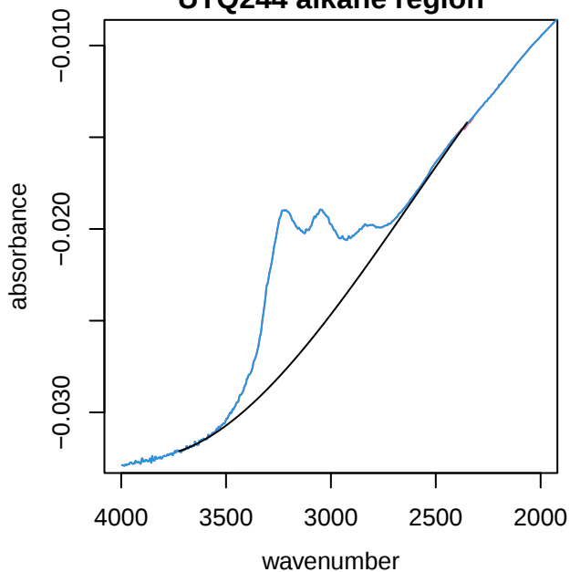
UTQ244 alkane region
