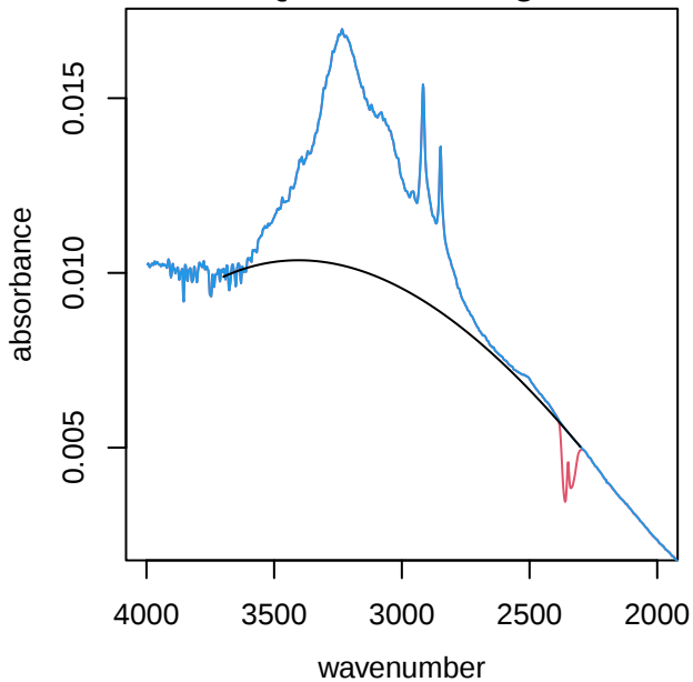
UTQ209 alkane region
