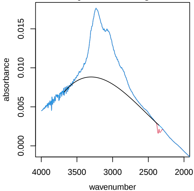
UTQ208 alkane region
