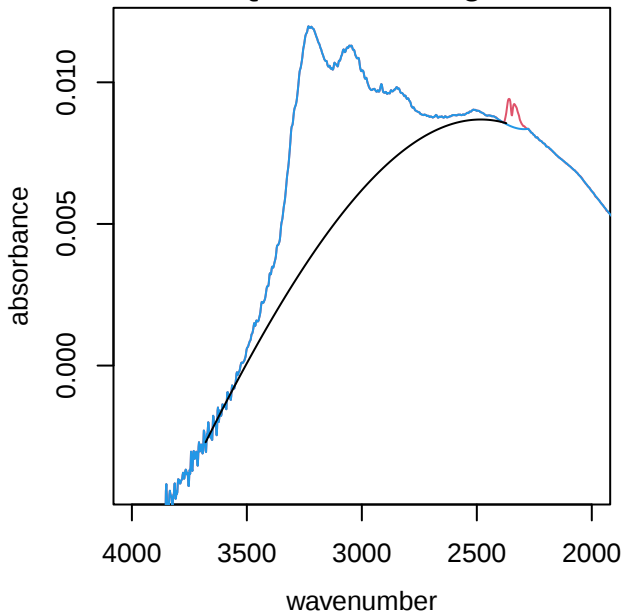
UTQ210 alkane region
