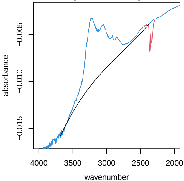
UTQ211 alkane region
