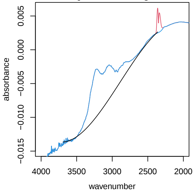
UTQ243 alkane region
