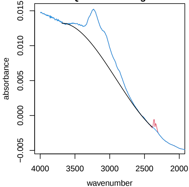
UTQ240 alkane region
