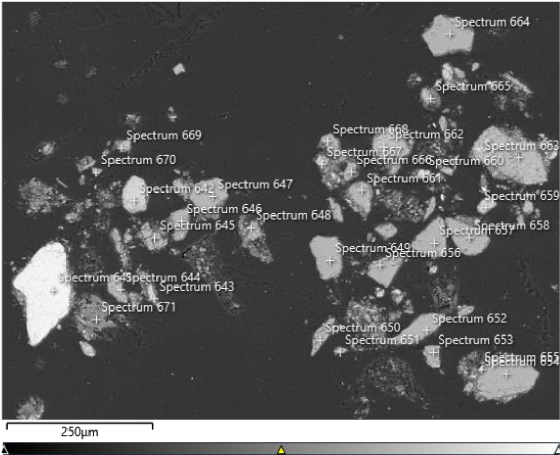
Electron Image 32
