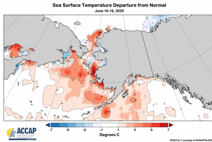
Figure 15b. 17 June sea surface temperature departures in the Alaska seas. Image courtesy of Richard Thoman, IARC/UAF.
