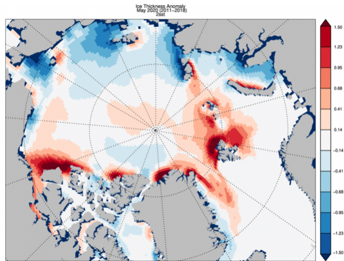
Figure 11. May 2020 sea-ice thickness anomaly (relative to 2011-2018). Figure courtesy of PIOMAS.
