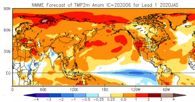
Figure 17. The outlook for summer temperature anomalies (C) based on the NMME forecasts for July–September 2020. Source: NOAA Climate Prediction Center.
