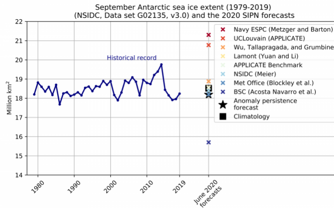
Figure 22. September Sea-ice Outlook for the Antarctic, together with the historical record based on NSIDC data set G02135, v3.0.
