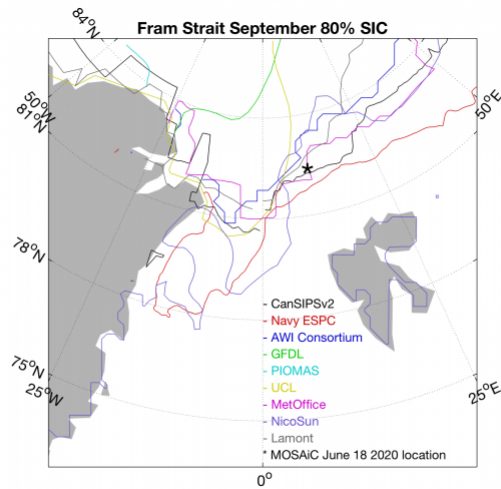
Figure 21a. Forecasts of the September 80% SIC contour, and the current location of the Polarstern/MOSAIC. Figure courtesy of Blanchard-Wrigglesworth
