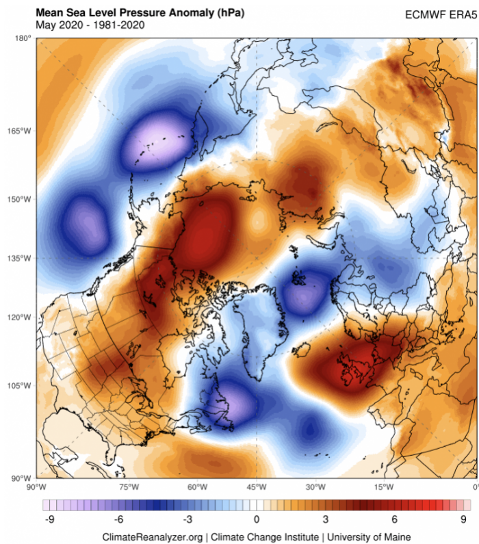
Figure 16. Sea level pressure anomalies during May 2020. From the Climate Reanalyzer.
