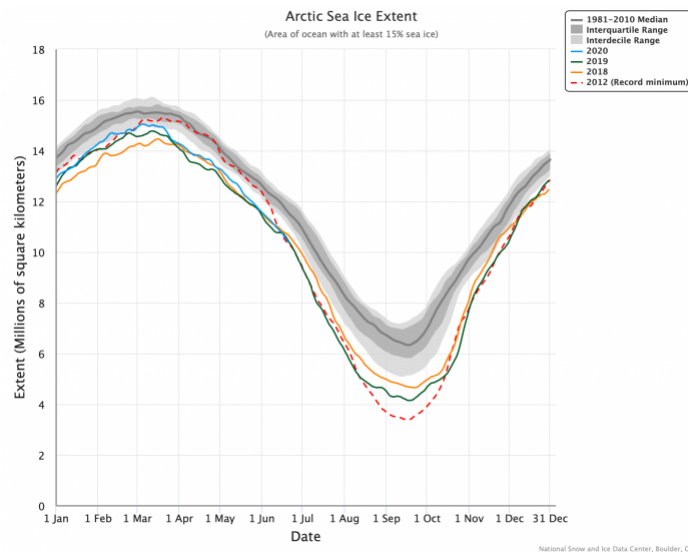
Figure 7. Time-series of Arctic sea-ice extent for 2020 and recent two years compared to 2012 and the climatology of 1981–2010. Figure courtesy of the National Snow and Ice Data Center.
