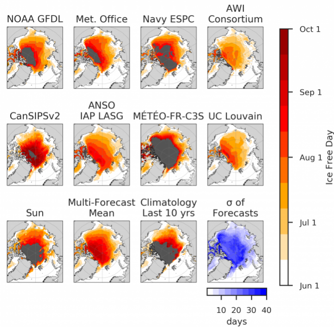
Figure 5b. First ice-free date forecasts for a 80% sea ice concentration threshold. The black region indicates where a location is forecasted to be above the threshold for all lead times. The standard deviations (last panel) indicate where contributions diverge. Figure courtesy of Bitz and Blanchard-Wrigglesworth. Updated on 4 August 2020.
