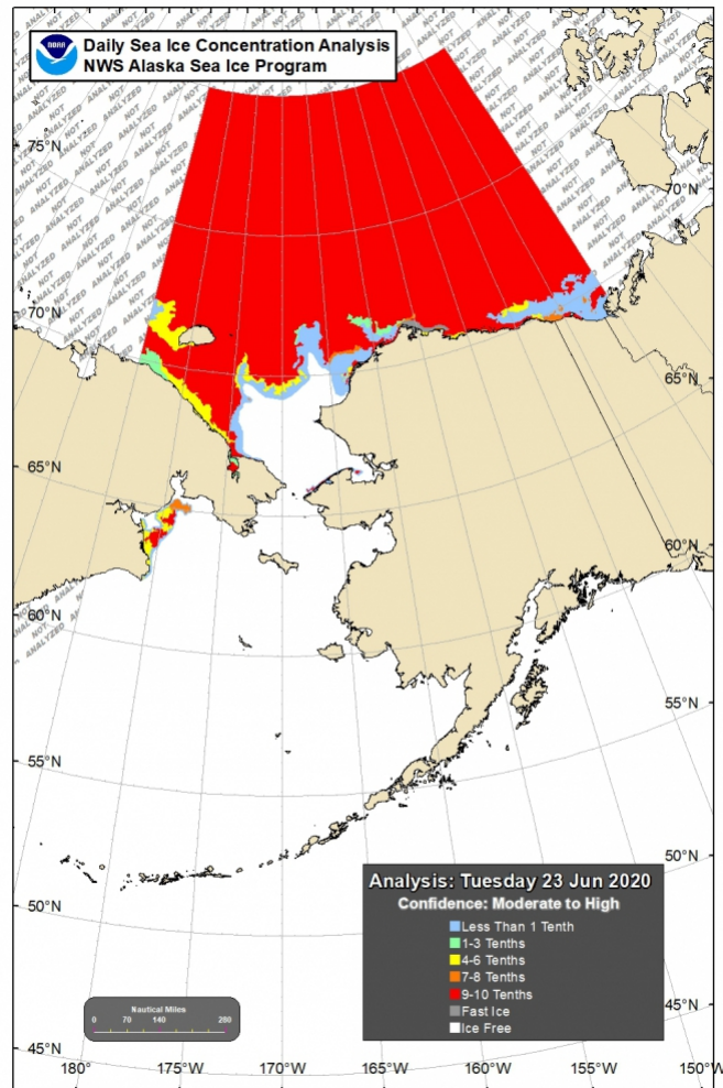
Figure 12. Sea-ice conditions for the northern Bering and Chukchi seas for mid-June. Sea ice retreated rapidly in early June from St. Lawrence Island in the Bering Sea all the way north well into the Chukchi Sea. Although the Bering Sea had a larger sea-ice extent in the winter and spring of 2020 relative to 2018 and 2019, thin ice in 2020 led to a rapid retreat. Figure courtesy of the NWS Anchorage Sea Ice Desk.
