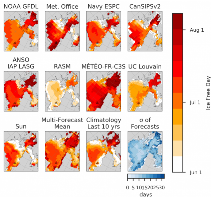
Figure 20a. First ice-free date (IFD) forecasts for a 15% sea ice concentration threshold for the Hudson Bay. The standard deviations (last panel) indicate where contributions diverge. Figure courtesy of Bitz and Blanchard-Wrigglesworth. Updated on 4 August 2020.
