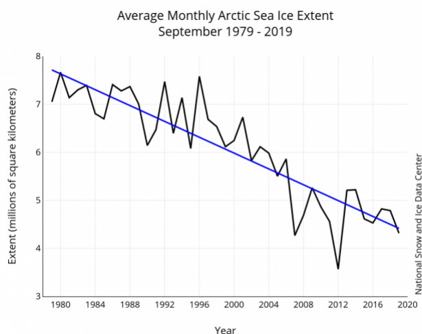
Figure 3. Historical data on Arctic September sea-ice extent. Image from National Snow and Ice Data Center (NSIDC).
