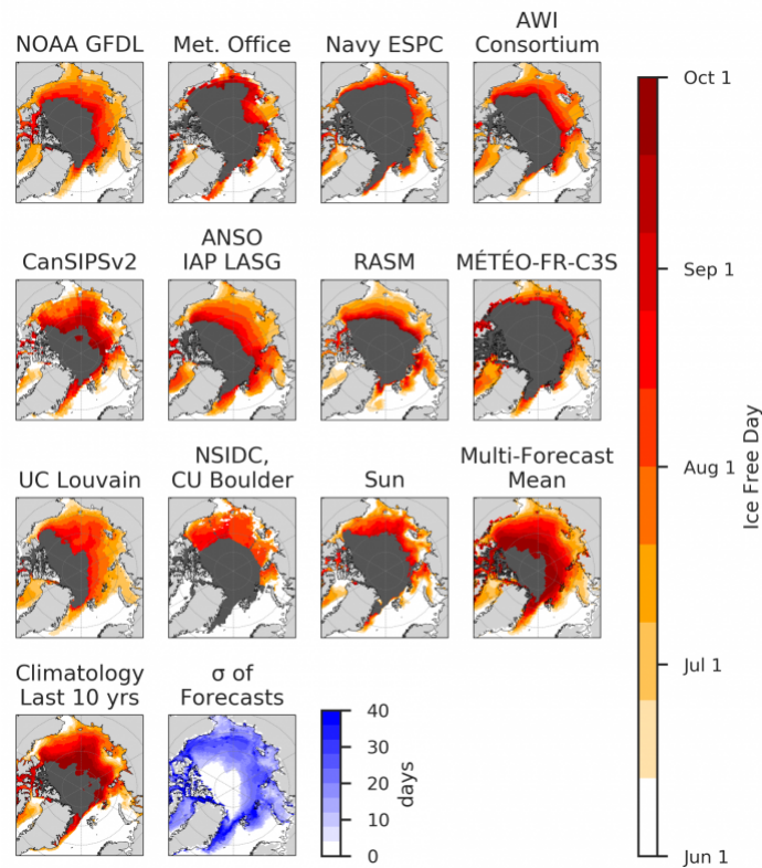
Figure 5a. First ice-free date forecasts for a 15% sea ice concentration threshold. The black region indicates where a location is forecasted to be above the threshold for all lead times. The standard deviations (last panel) indicate where contributions diverge. Figure courtesy of Bitz and Blanchard-Wrigglesworth. Updated on 4 August 2020.
