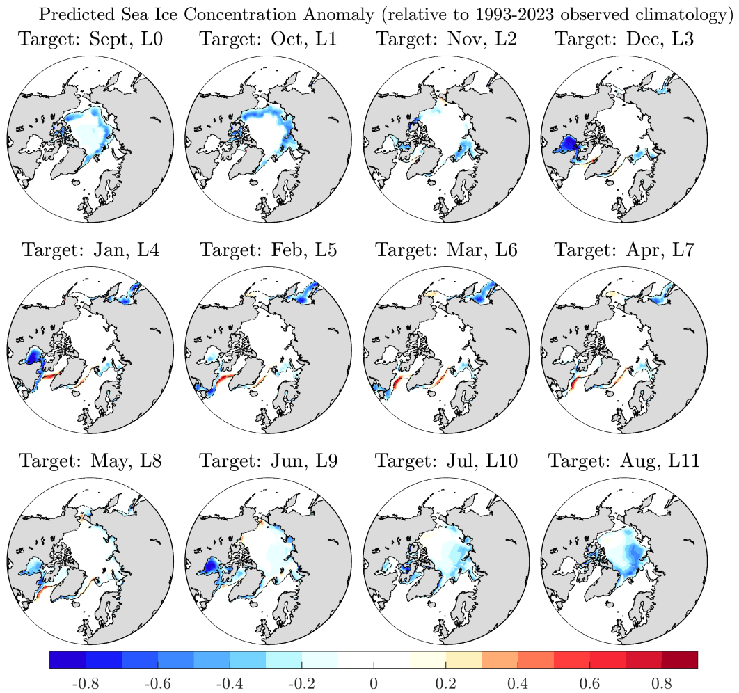
Figure 4: Monthly sea ice concentration anomaly predictions from the GFDL-SPEAR_MED model initialized on September 1. The anomalies are computed relative to the observed NSIDC SIC CDR climatology over 1993–2023. The observed climatological sea ice edge position is shown in black. No bias correction has been applied.
