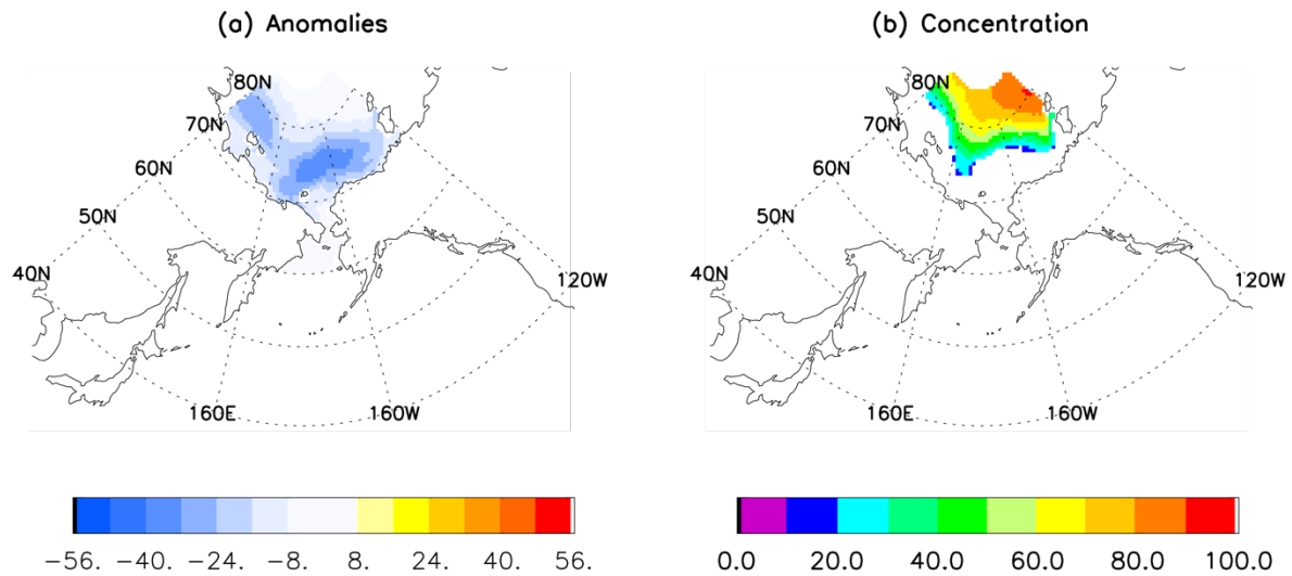
Figure 2 Two-month lead prediction of September 2024 sea ice concentration anomaly (a) and concentration (b) in the Alaskan region by a linear Markov model initialized with observed July SIC, SST, SAT, GPH and winds at 300mb.
