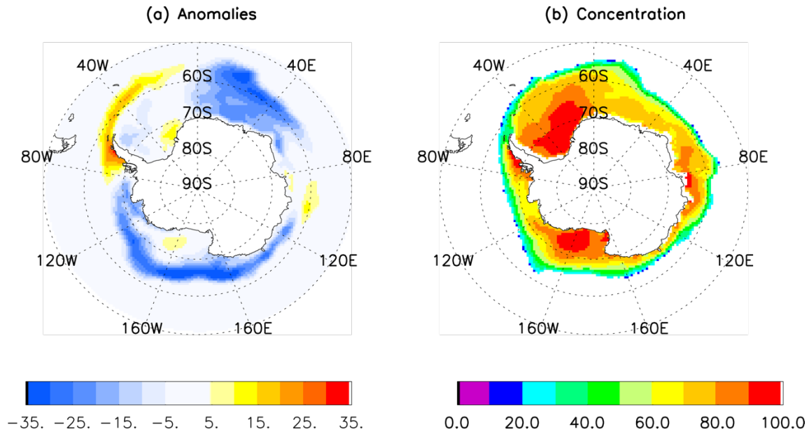
Figure 3 Two-month lead prediction of September 2024 Antarctic sea ice concentration anomaly (a) and concentration (b) by a linear Markov model initialized with observed July SIC, SST and SAT.
