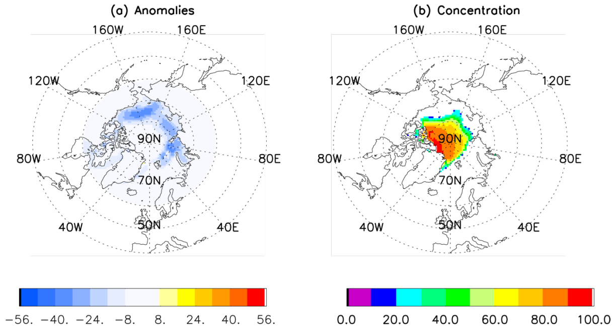
Figure 1 Two-month lead prediction of 2024 September Arctic sea ice concentration anomaly (a) and concentration (b) by the linear Markov model initialized with observed July SIC, SST, SAT, GH300 and vector winds at 300mb.
