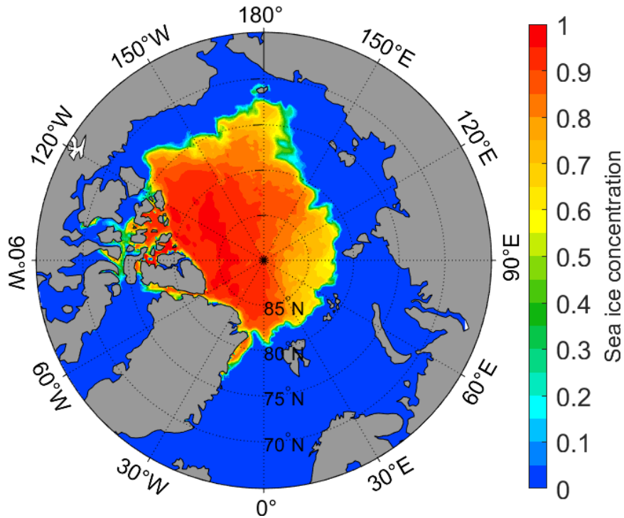
Figure s1. Spatial pattern of the predicted September-mean sea ice concentration (SIC).
