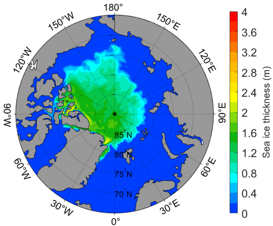
Figure s2. Spatial pattern of the predicted September-mean sea ice thickness (SIT).
