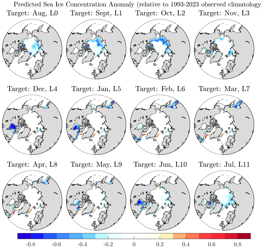
Figure 4: Monthly sea ice concentration anomaly predictions from the GFDL-SPEAR_MED model initialized on August 1. The anomalies are computed relative to the observed NSIDC SIC CDR climatology over 1993–2023. The observed climatological sea ice edge position is shown in black. No bias correction has been applied.
