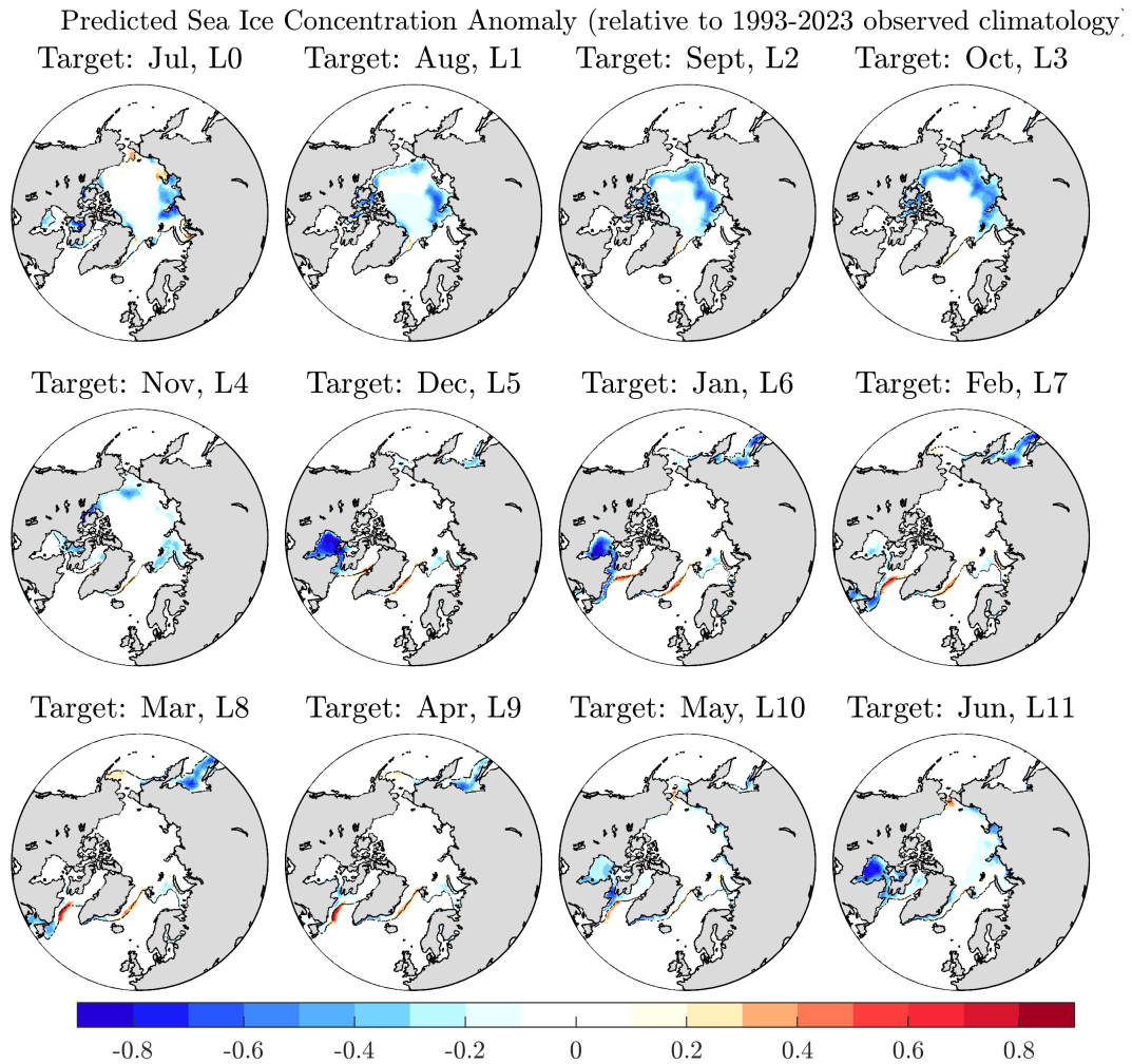
Figure 4: Monthly sea ice concentration anomaly predictions from the GFDL-SPEAR_MED model initialized on July 1. The anomalies are computed relative to the observed NSIDC SIC CDR climatology over 1993–2023. The observed climatological sea ice edge position is shown in black. No bias correction has been applied.
