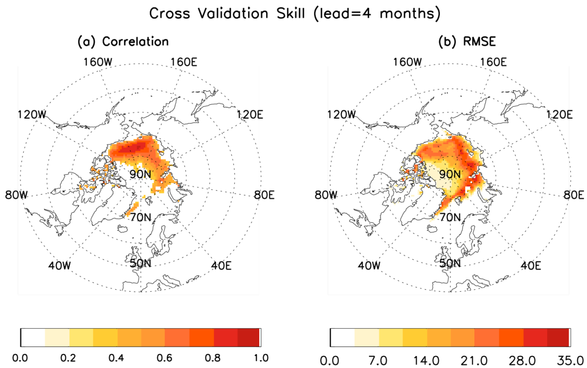
Figure 4. Cross-validated model skill measured by correlations between model predictions and observations of Arctic sea ice concentration anomalies (a) and model RMSE (b) for four-month
