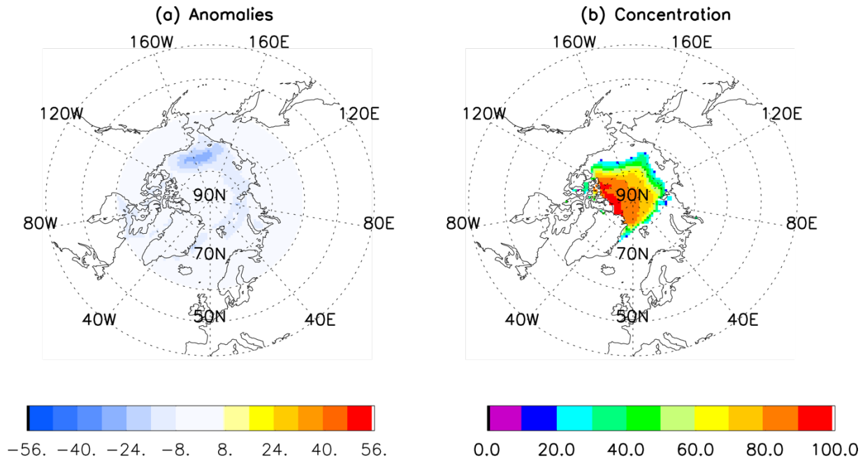
Figure 1 Four-month lead prediction of 2024 September Arctic sea ice concentration anomaly (a) and concentration (b) by the linear Markov model initialized with observed May SIC, SST, SAT, GH300 and vector winds at 300mb.
