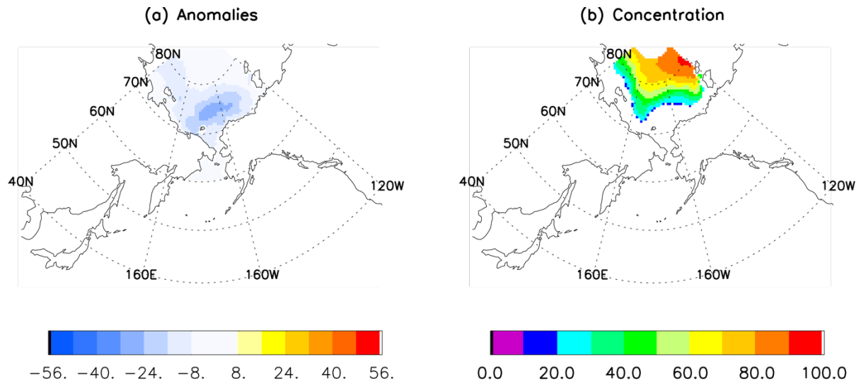
Figure 2 Four-month lead prediction of September 2024 sea ice concentration anomaly (a) and concentration (b) in the Alaskan region by a regional linear Markov model initialized with observed May SIC, SST, and SAT.
