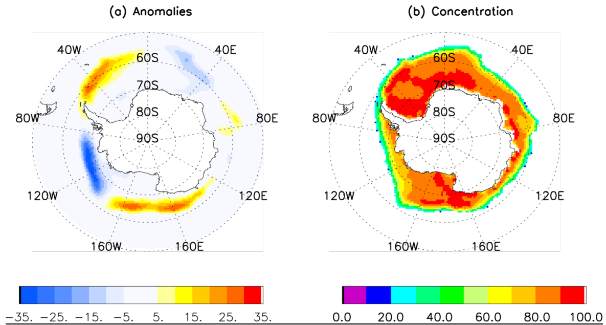
Figure 3 Four-month lead prediction of September 2024 Antarctic sea ice concentration anomaly (a) and concentration (b) by a linear Markov model initialized with observed May SIC, SST and SAT.
