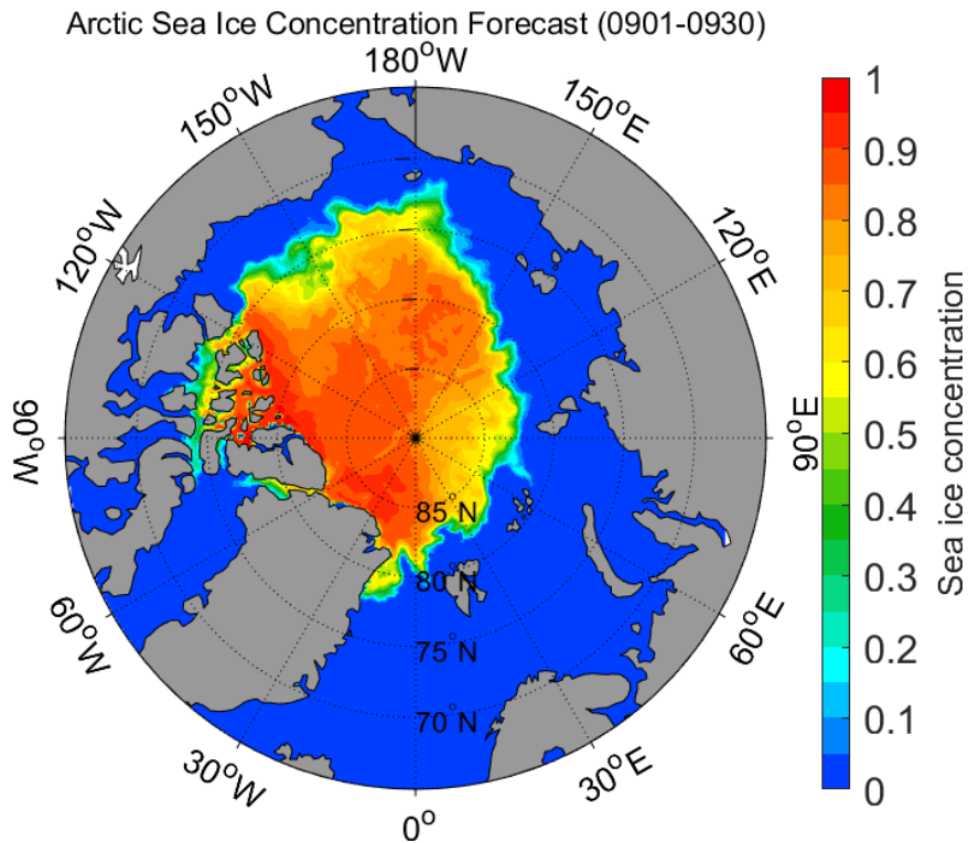
Figure s1. Spatial pattern of the predicted September-mean sea ice concentration (SIC).
