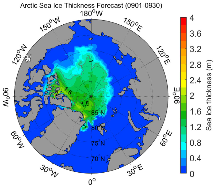
Figure s2. Spatial pattern of the predicted September-mean sea ice thickness (SIT).
