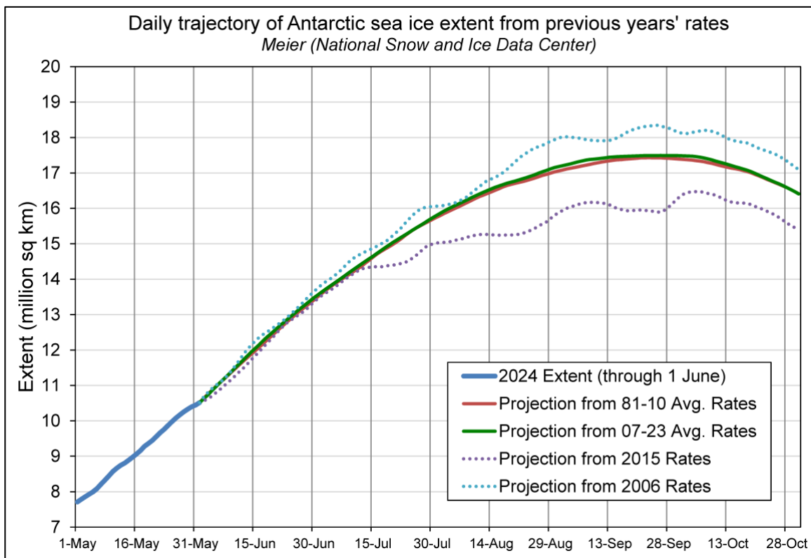
Figure 2. Predicted Antarctic trajectories from the 1 June observed extent. The official estimate is based on the projection used the average of the last 17 years (2007-2023, green solid line) and for the 1981-2010 average (solid red line). The rates for 2006 and 2015 (dotted lines) yield the highest and lowest predicted extents respectively.
