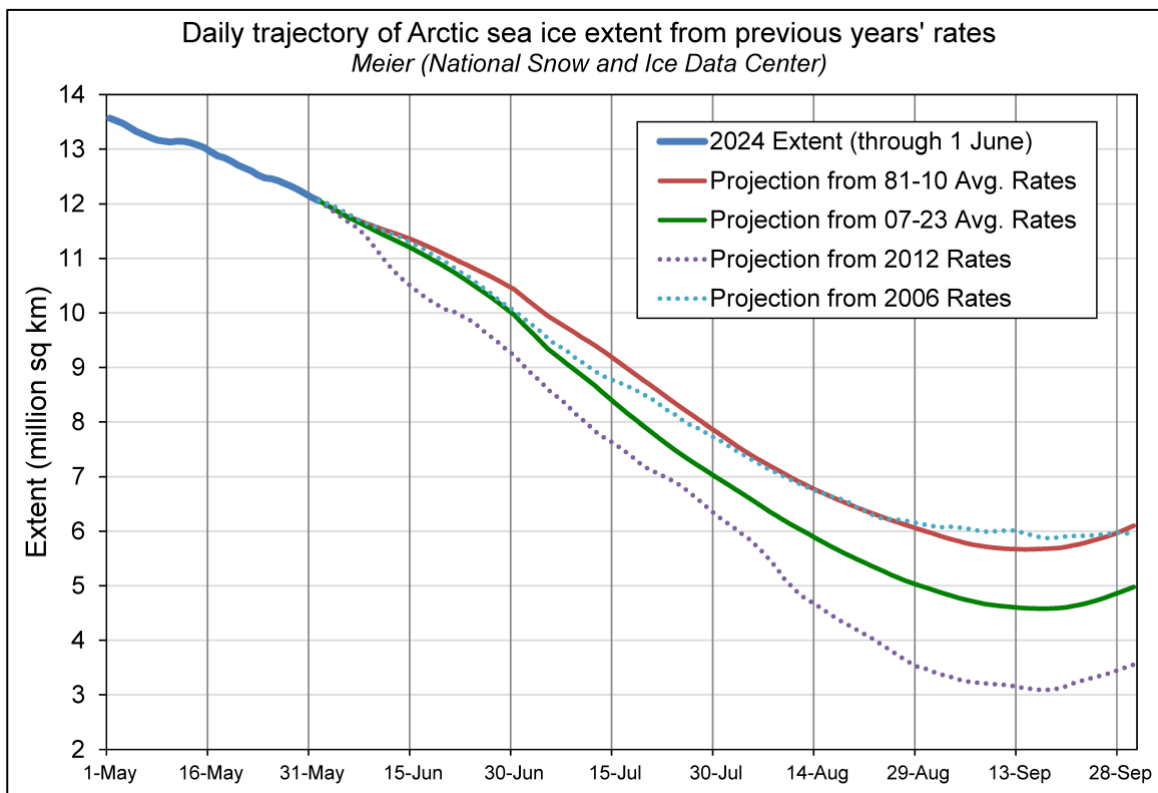
Figure 1. Predicted Arctic trajectories from the 1 June observed extent. The official estimate is based on the projection used the average of the last 17 years (2007-2023, green solid line) and for the 1981-2010 average (solid red line). The rates for 2006 and 2012 (dotted lines) yield the highest and lowest predicted extents respectively.
