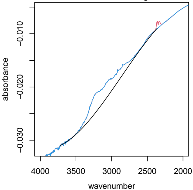
UTQ228 alkane region
