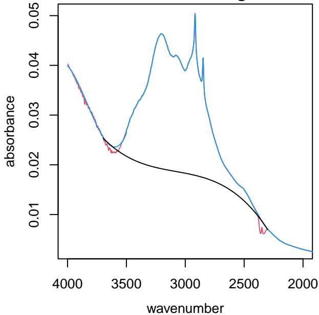
UTQ226 alkane region
