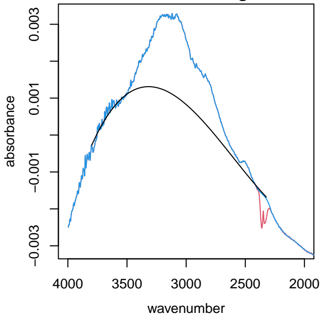
UTQ289 alkane region
