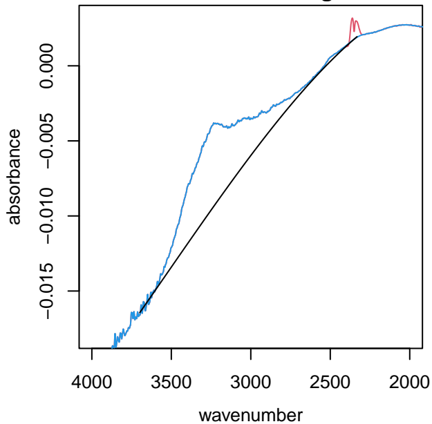
UTQ288 alkane region
