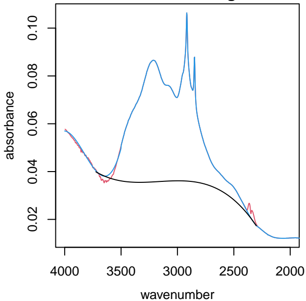
UTQ227 alkane region
